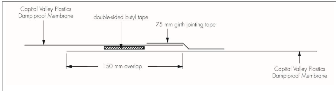
Figure 1 Double-sided butyl tape joint
