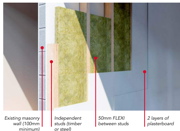
Figure 12 Acoustic applications – separating walls
