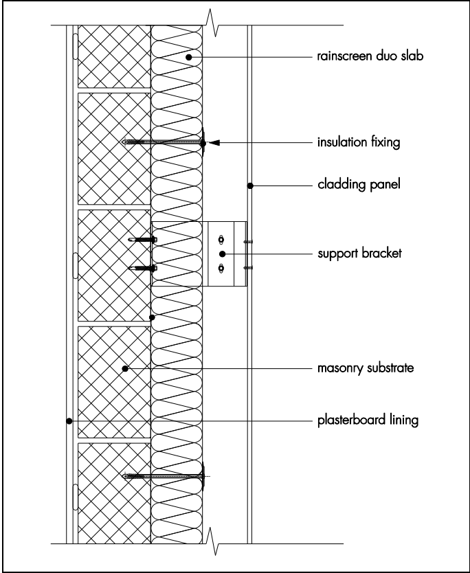
Figure 3 Masonry substrate
