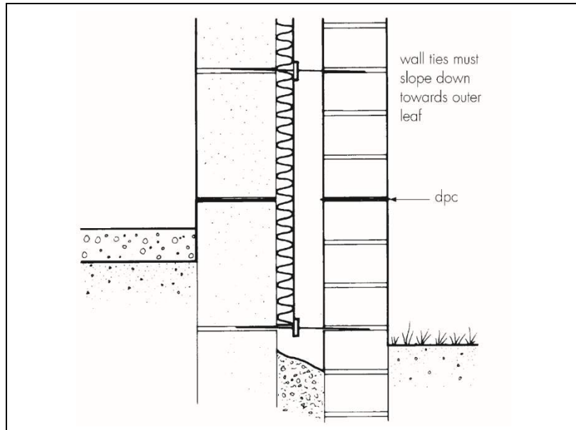
Figure 2 Detail of wall ties
