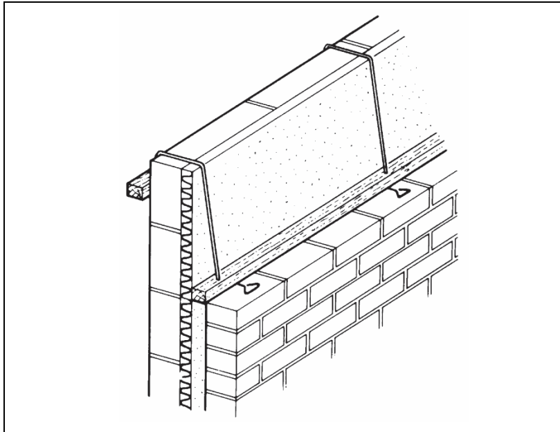
Figure 3 Use of cavity batten
