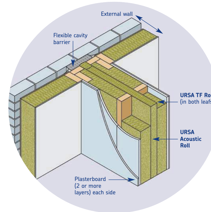
Figure 5 – Timber Frame Separating/External Wall Junction
