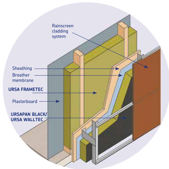
Figure 4 – Rainscreen Cladding on Timber Framed Wall
